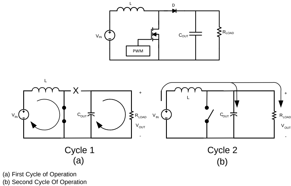
Figure 56. Simplified Boost Converter Diagram
